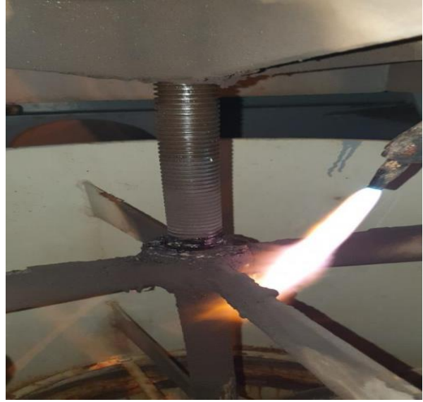
Having checked the situation, we found that the grease residues has hardened and we carry out heating on the cargo hold flap spindle and found to be succesful
