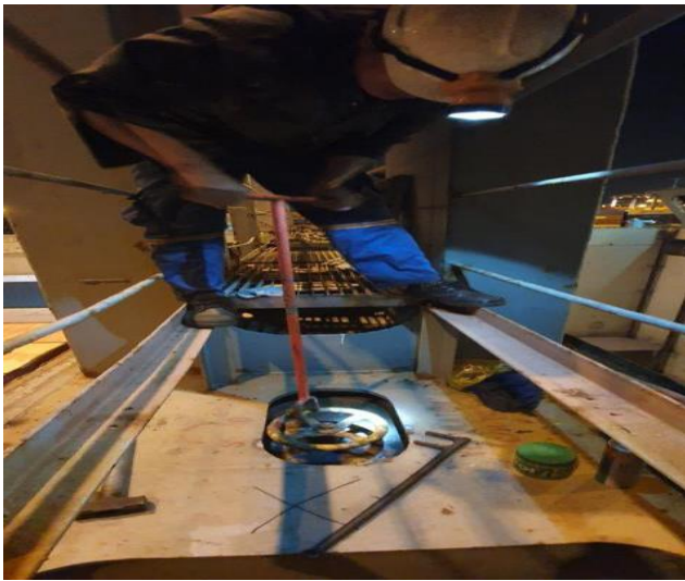
Having checked the situation, we found that the grease residues has hardened and we carry out heating on the cargo hold flap spindle and found to be succesful
